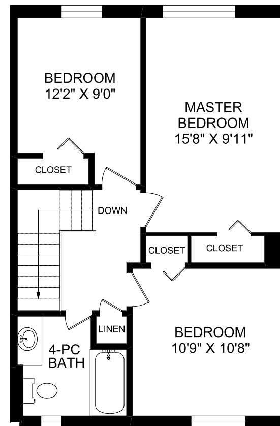
SECOND LEVEL
