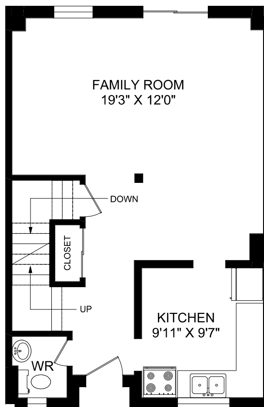
MAIN LEVEL
