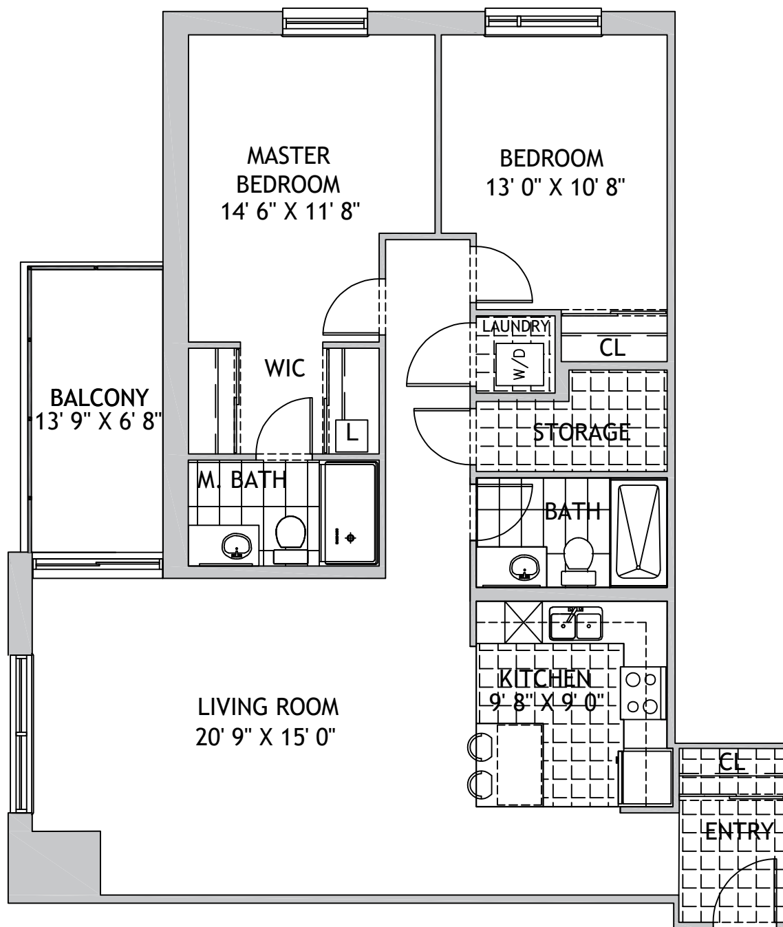
Typical Floor Layout
