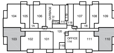
Ground Floor Plan Typical Floor Layout
