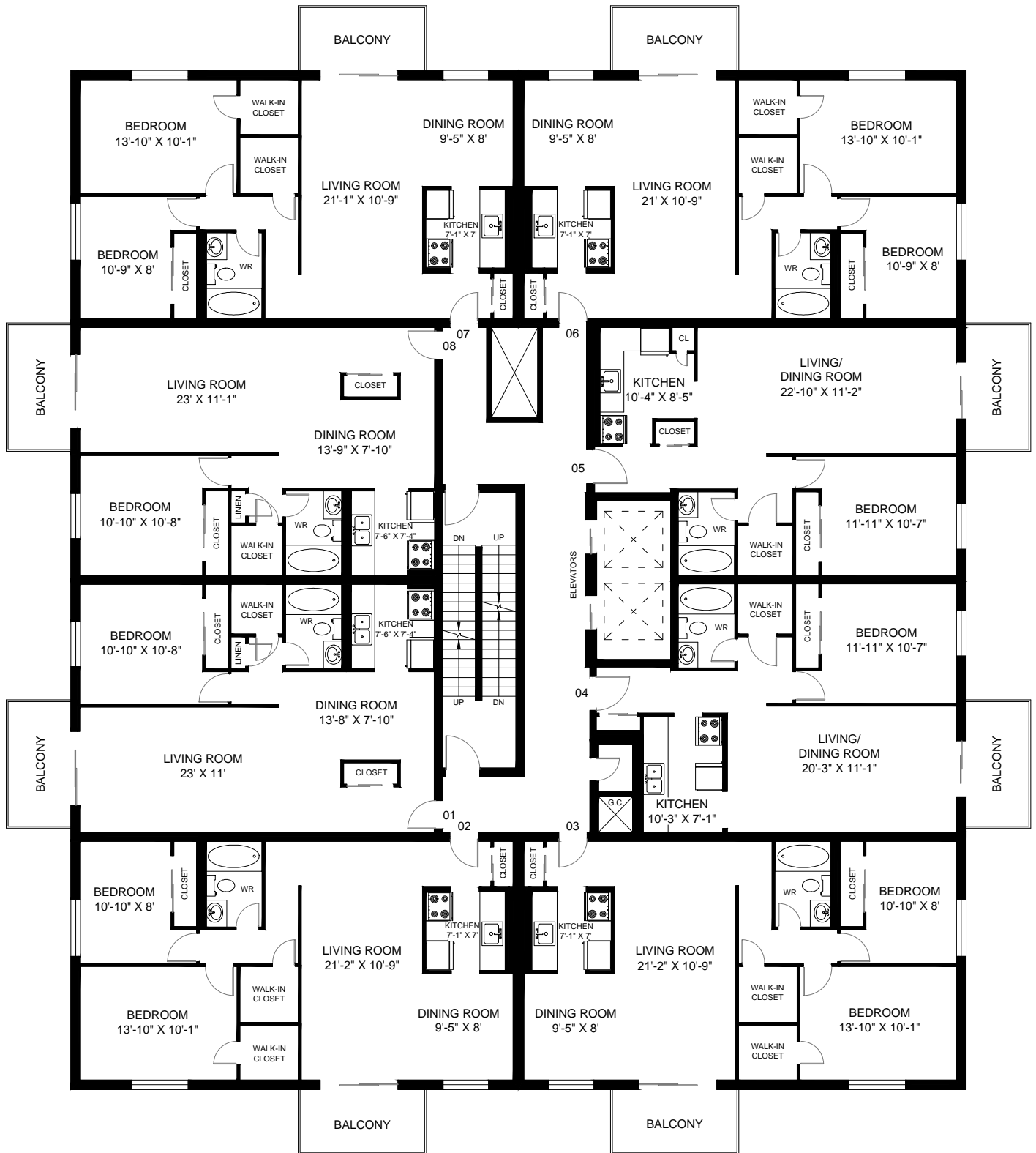
TYPICAL FLOOR (2ND - 11TH) PLAN
