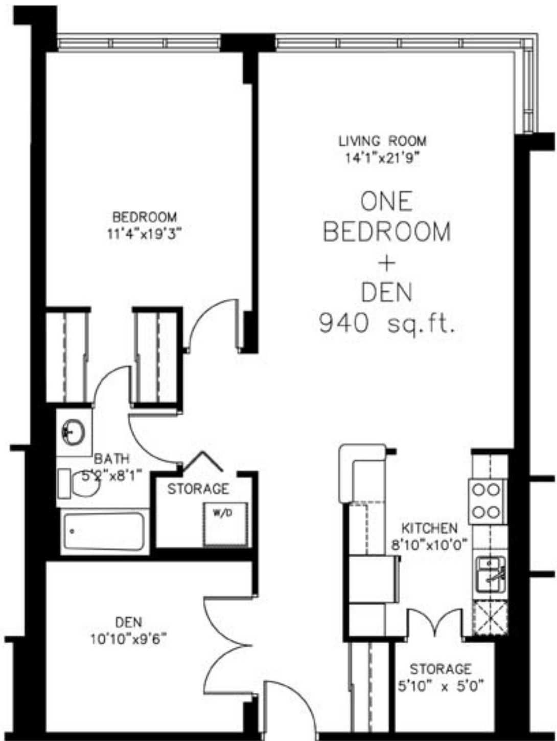
TYPICAL PLAN FLOORS 4-14
