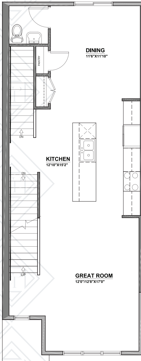
MAIN FLOOR (LEVEL 3) 788 SQ. FT.
